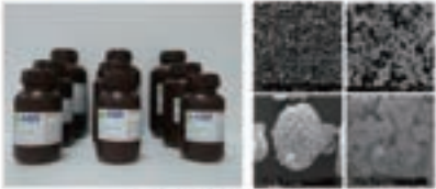
NMC532, NMC622
